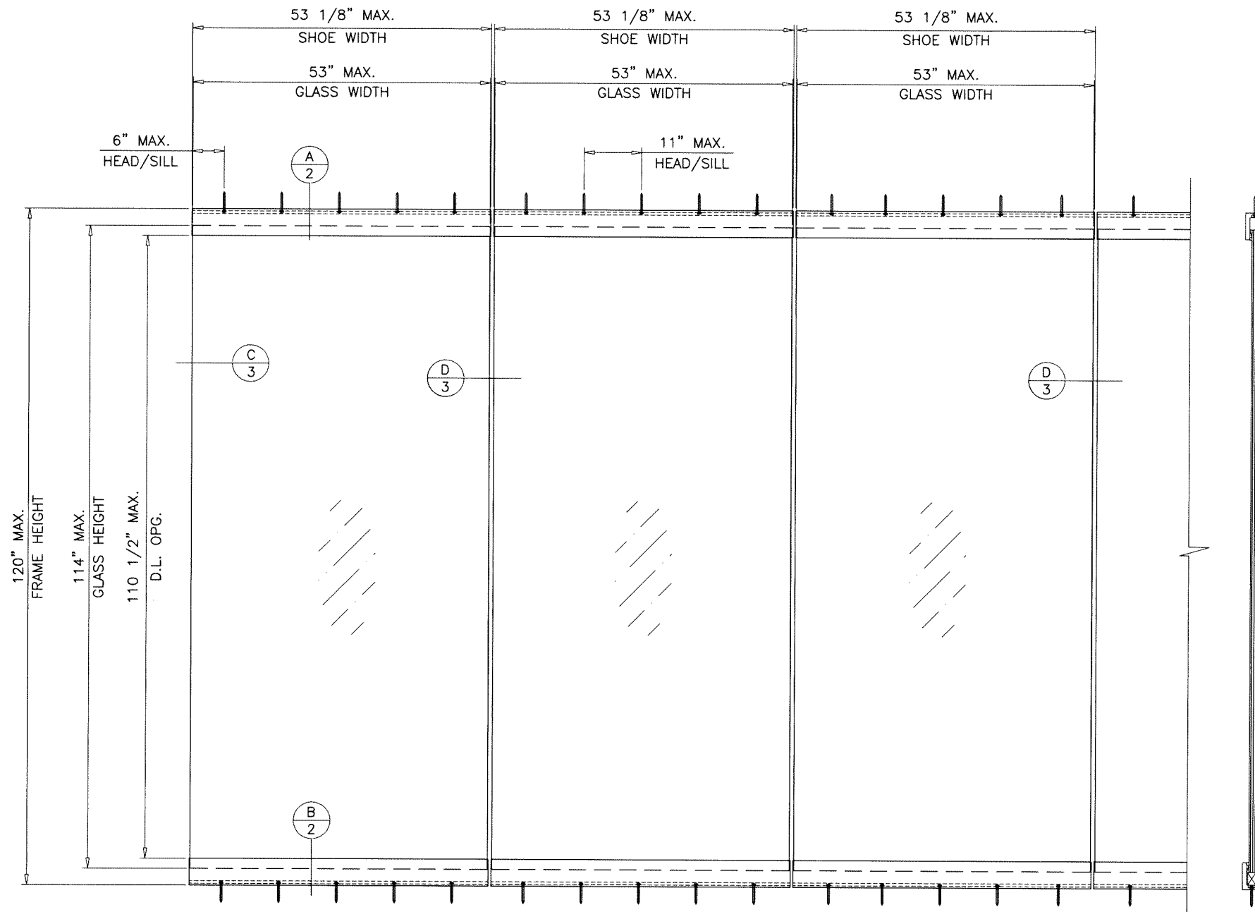
TYPICAL ELEVATION
